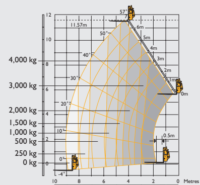
540-170 Stabilisers retracted
